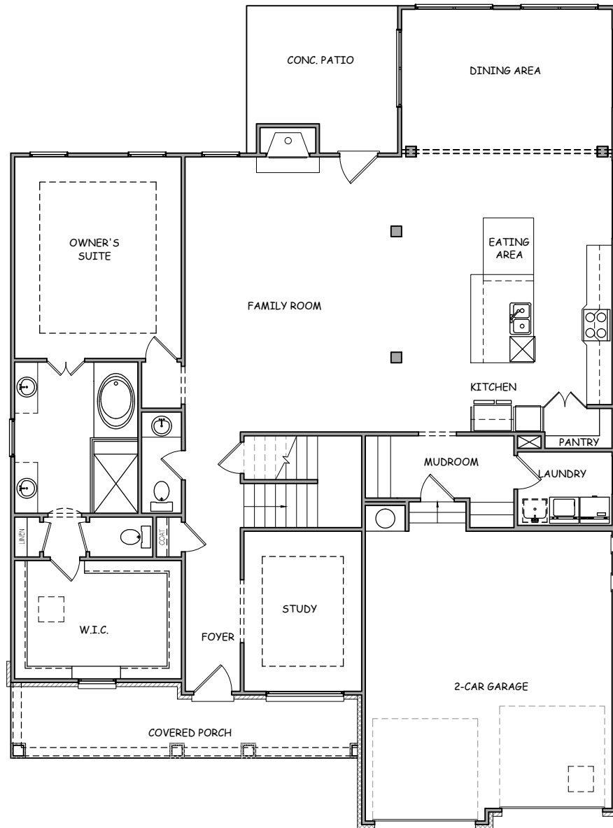
FIRST FLOORPLAN
